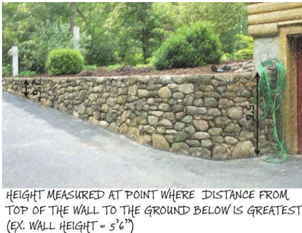
Figure 3-05. Retaining Wall Height
